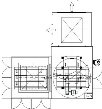
PI Post Bake Layout
